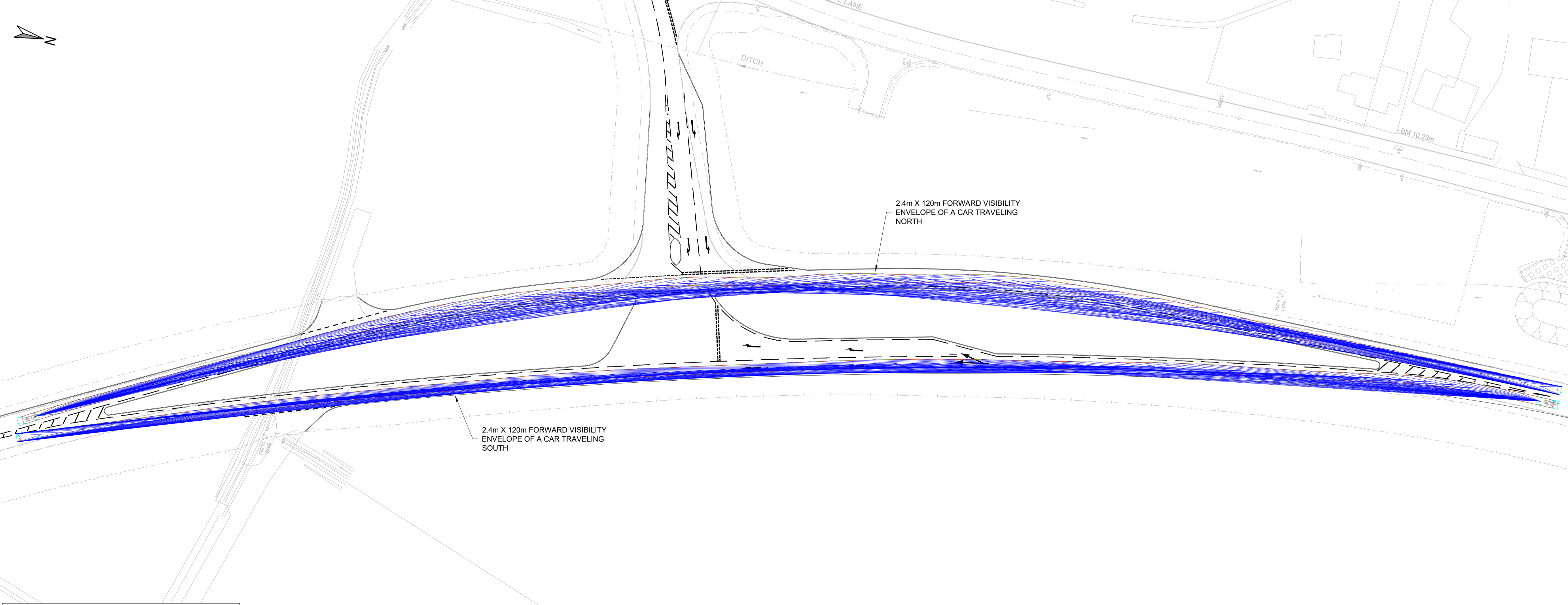
TITLE: LARGE CAR FORWARD VISIBILITY ENVELOPE
